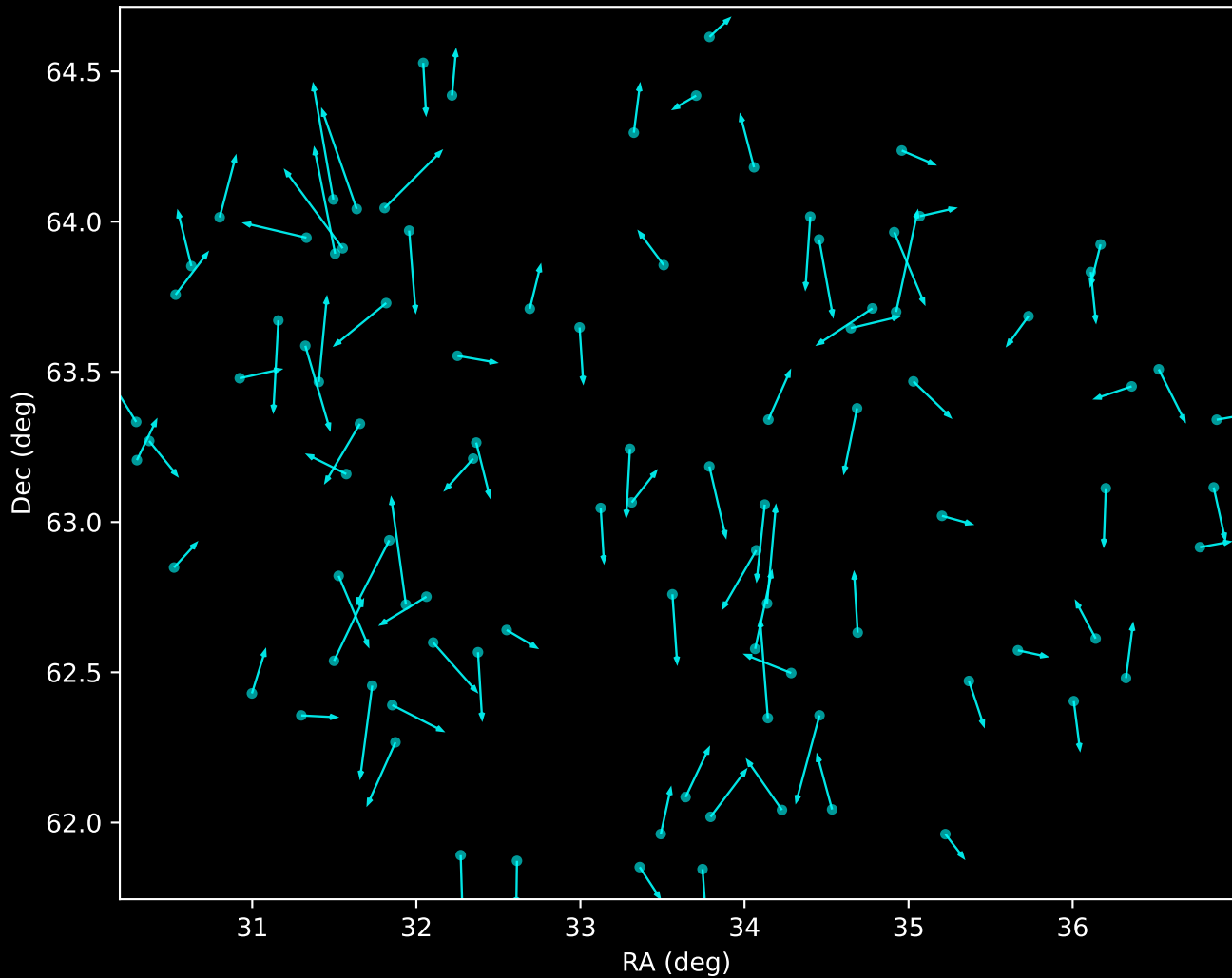
APOGEE DR17 Noise Stream Proper Motion Vectors (n=95)
