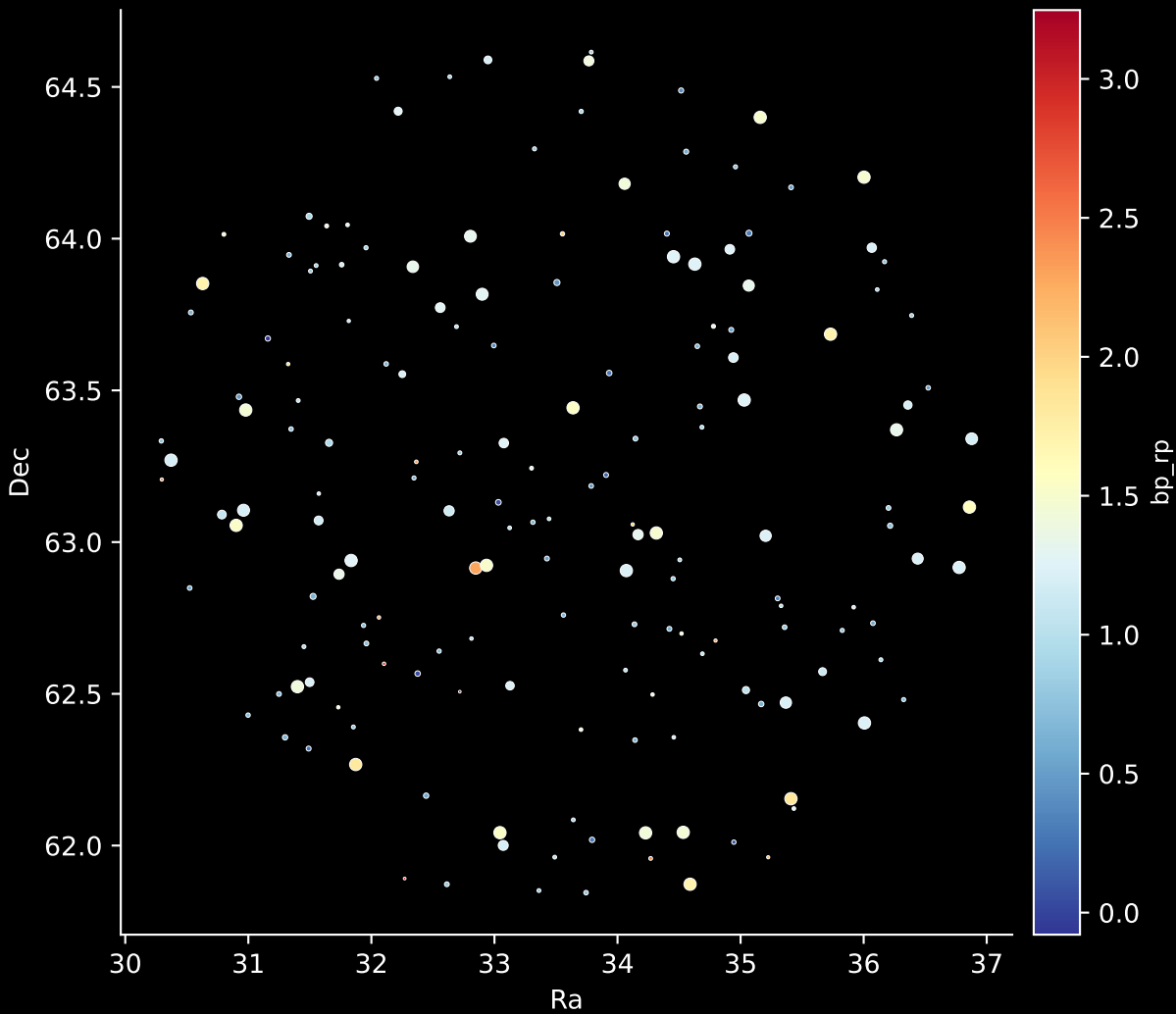
APOGEE DR17 Field: [CVZTILE_095+19_btx] Stars: 169
