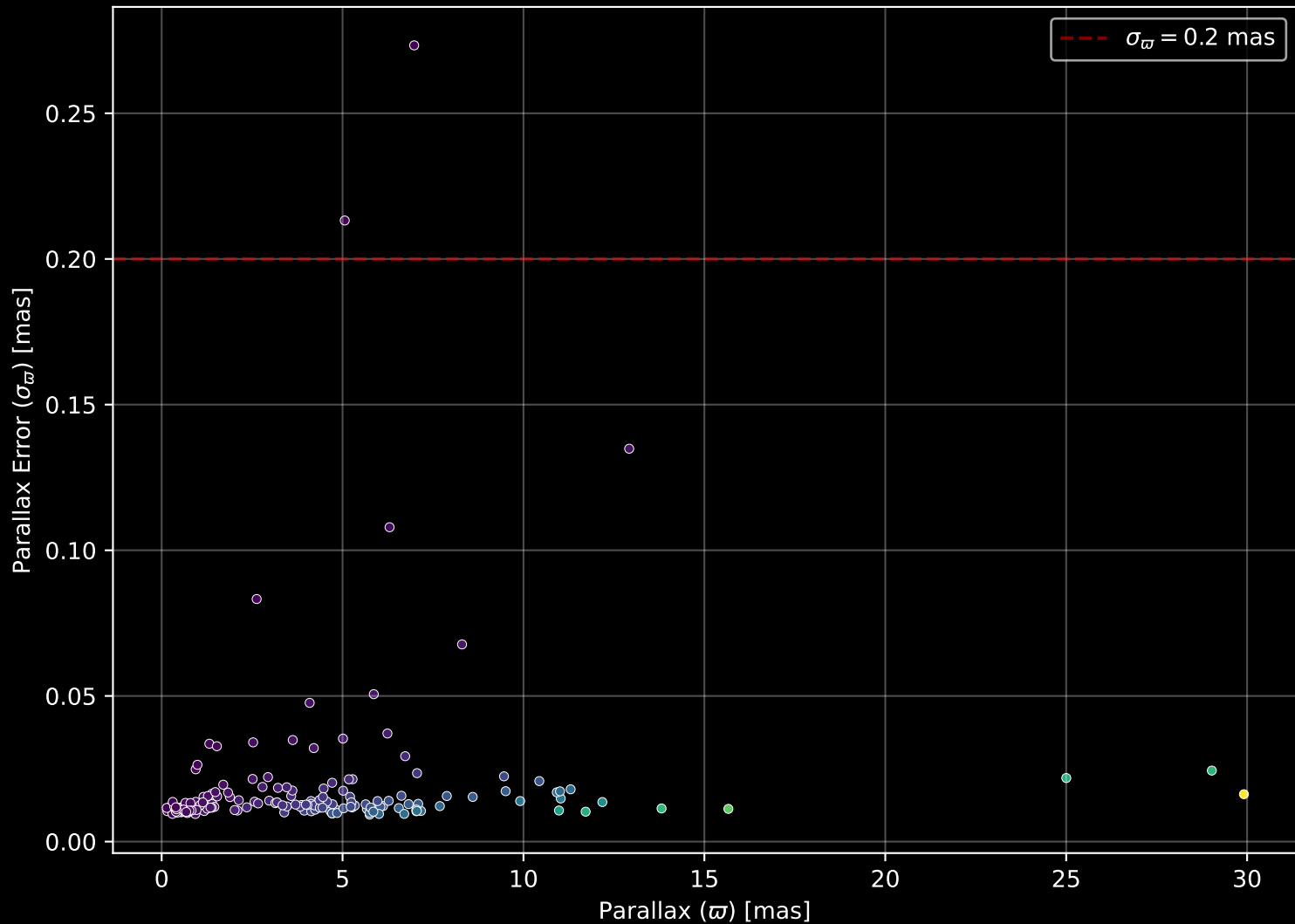
APOGEE DR17 Field: [CVZTILE_095+19_btx] Parallax Quality (n= 169)
