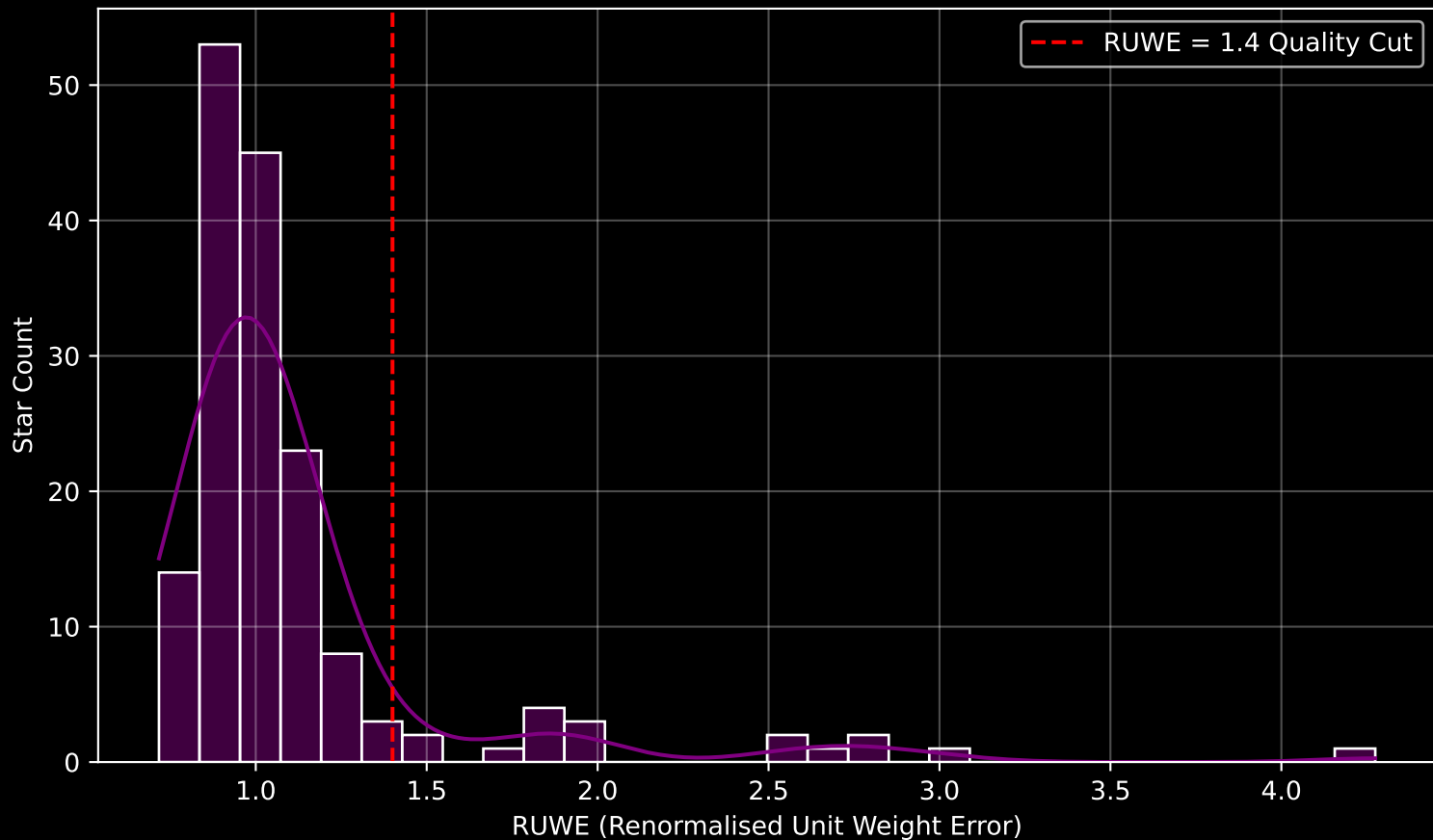
GAPOGEE DR17 Field [CVZTILE_095+19_btx] RUWE Distribution (n= 163)
