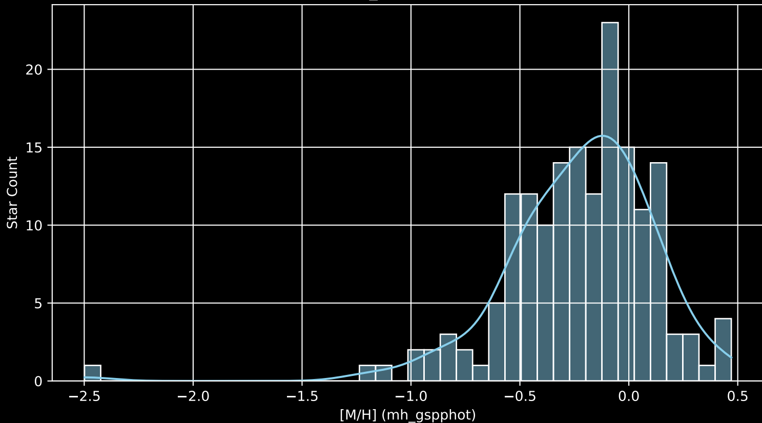
APOGEE DR17 Field: [CVZTILE_095+19_btx [M/H] (mh_gspphot) (n= 167)
