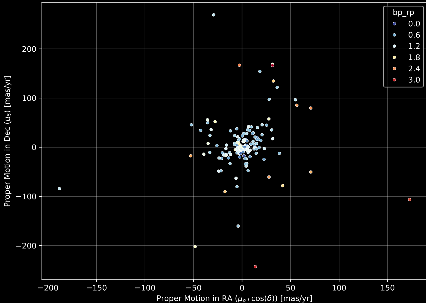
APOGEE DR17 Field: [CVZTILE_095+19_btx] Proper Motion Diagram (n= 169)
