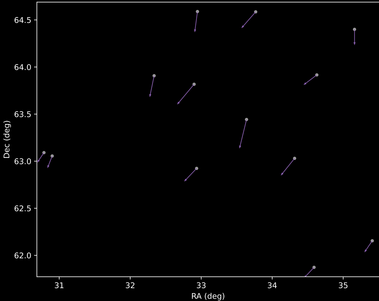
APOGEE DR17 Cluster 8 Proper Motion Vectors (n=13)
