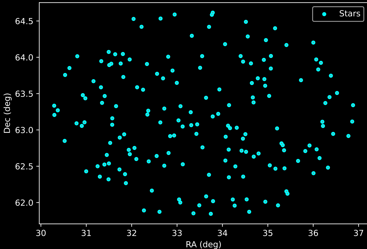
APOGEE DR17 Field: [CVZTILE_095+19_btx] Proper Motion Vectors for Gaia Star Field ( n = 169 )
