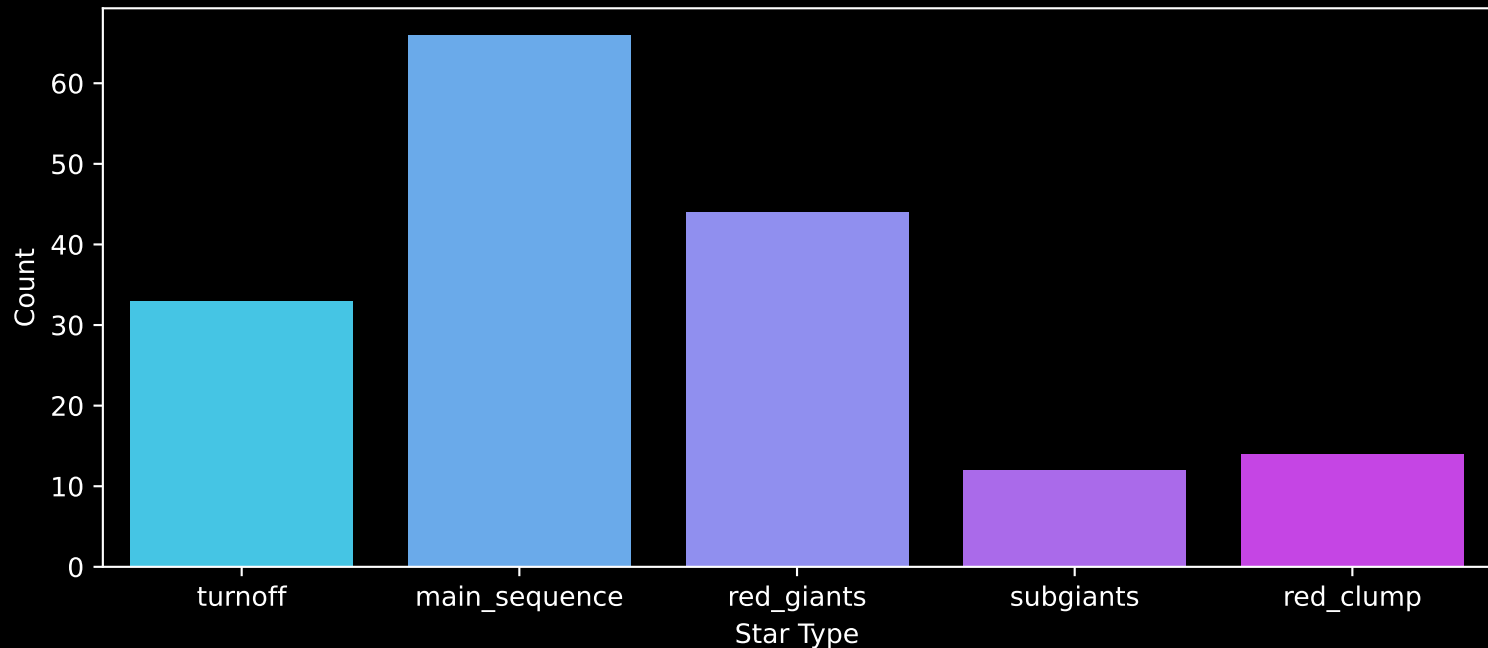
APOGEE DR17 Field: [CVZTILE_095+19_btx] Count plot of Star Type
